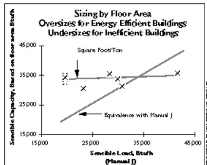
Figure 5. Sizing by house floor area.
