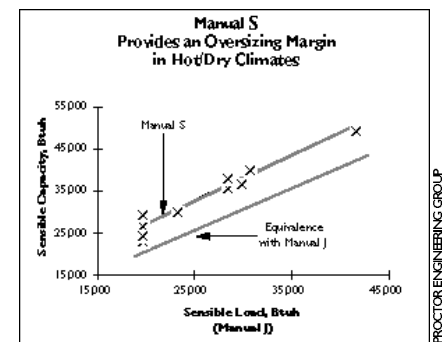
Figure 6. Manual S selection from Manual J loads.
